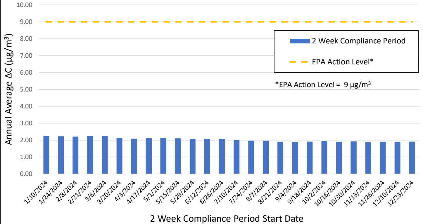
BENZENE FENCELINE ROLLING ANNUAL AVERAGE CONCENTRATION 01/10/2024 - 01/07/2025
